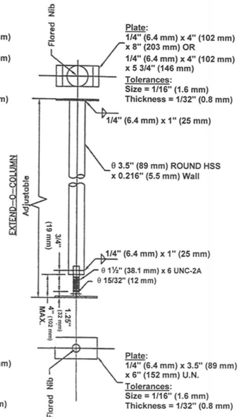
Figure 3 - Adjustable Length Column
