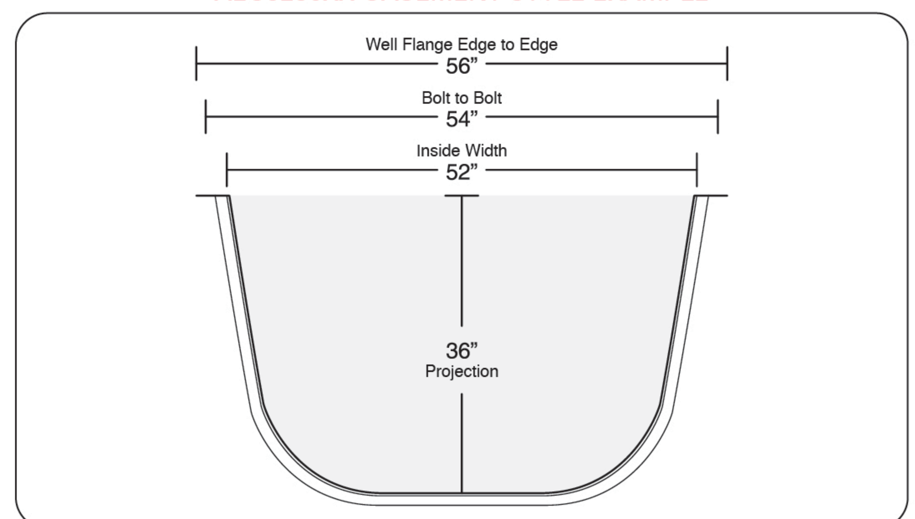
AEC5236XX CASEMENT STYLE EXAMPLE
