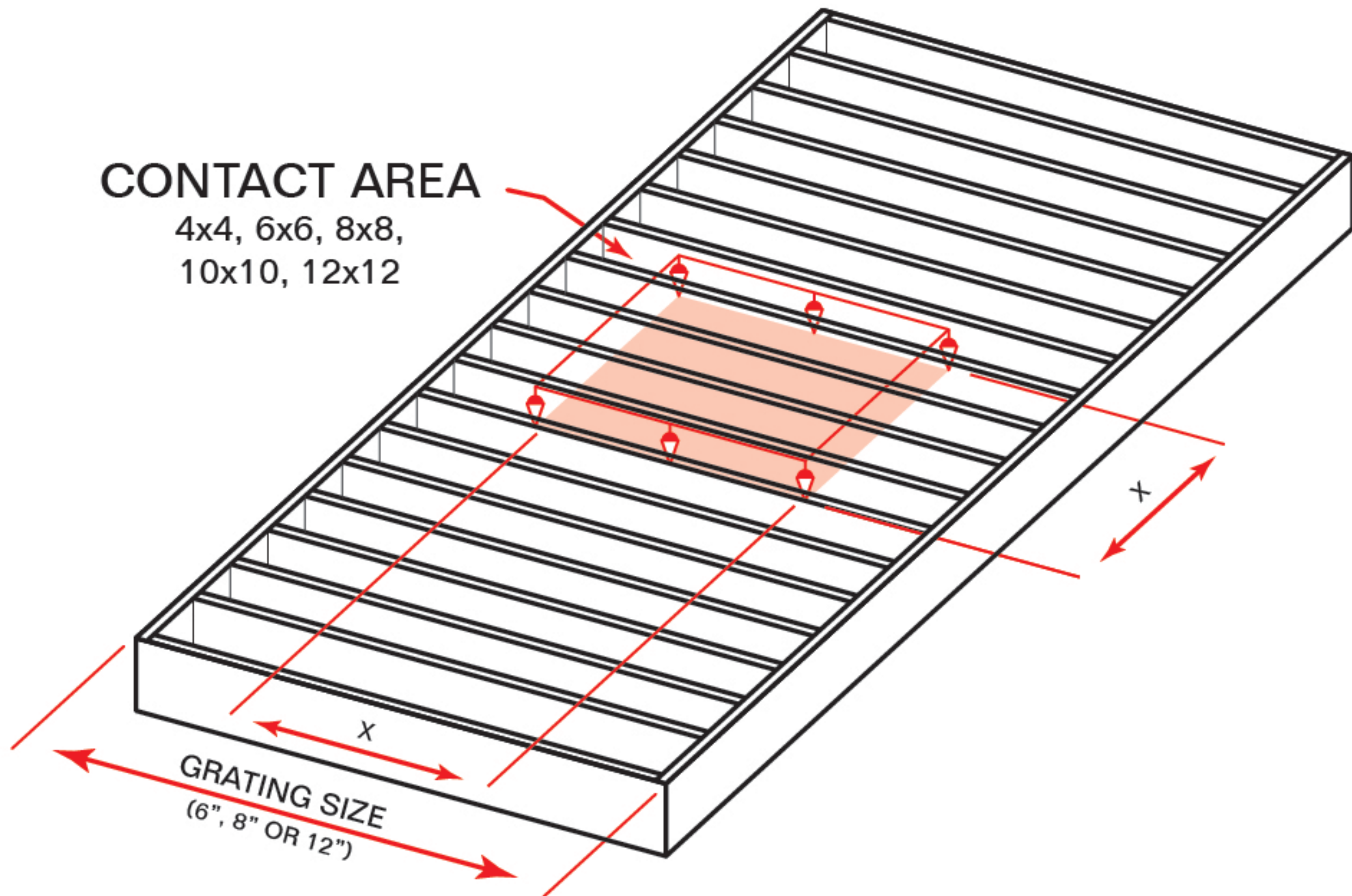
Welded Grating
