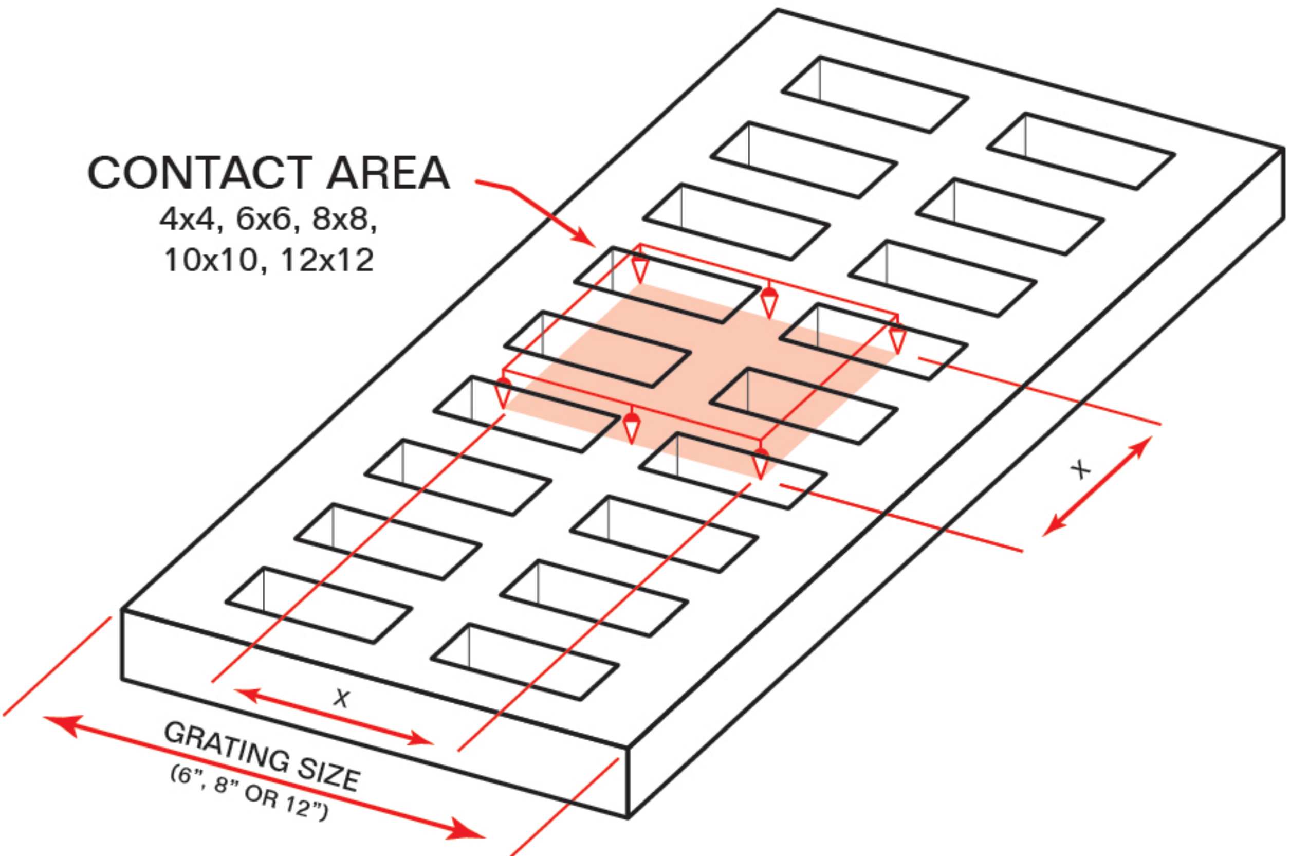
Cast Grating
